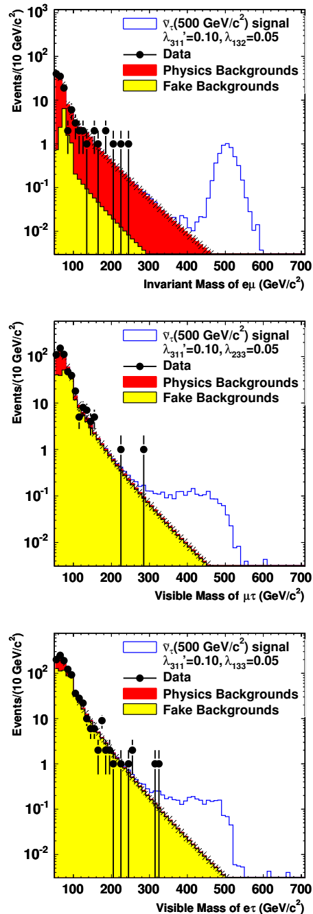
FIG. 1: Expected SM and observed distributions in M_{\text{ll}} for e\mu , \mu\tau and e\tau channels. Also shown is an expected \tilde{\nu}_\tau signal for M_{\tilde{\nu}_\tau} = 500 \text{ GeV}/c^2 and RPV couplings \lambda'_{311} = 0.10 and \lambda_{i3k} = 0.05 .
