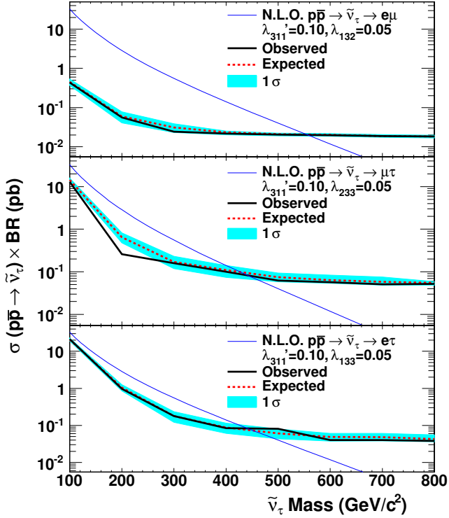
FIG. 2: The expected and observed 95% C.L. upper limits on \sigma(p\bar{p} \rightarrow \tilde{\nu}_\tau) \times \text{BR}(\tilde{\nu}_\tau \rightarrow e\mu/\mu\tau/e\tau) as a function of M_{\tilde{\nu}_\tau} .
