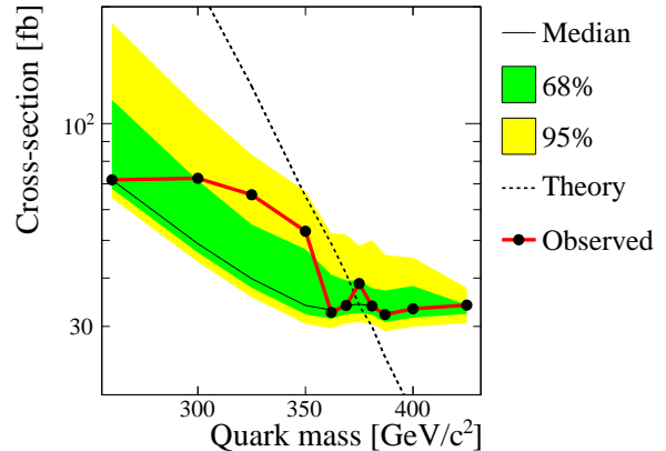
FIG. 2: Upper limits on b' production cross section at 95% C.L. assuming \mathcal{B}(b' \rightarrow Wt)=100\% . Solid black line is the median expected upper limit in simulated experiments without b' signal; green and yellow bands represent 68% and 95% of simulated experiments, respectively; solid red line is the observed limit. Dashed black line is the NLO b' production cross section [28, 29].
