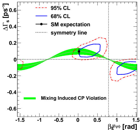
FIG. 16. (color online). Confidence regions in \beta_s^{J/\psi\phi} - \Delta\Gamma_s plane for the fit including flavor tagging information. The solid (blue) and dot-dashed (red) contours show the 68% and 95% confidence regions, respectively. The dotted lines are the symmetry axes corresponding to the profiled likelihood invariance under \beta_s^{J/\psi\phi} \rightarrow \frac{\pi}{2} - \beta_s^{J/\psi\phi} and \Delta\Gamma_s \rightarrow -\Delta\Gamma_s . The shaded (green) band is the theoretical prediction of mixing-induced CP violation.
