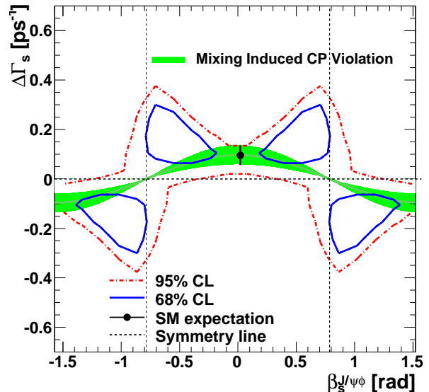
FIG. 15. (color online). Confidence regions in \beta_s^{J/\psi\phi} - \Delta\Gamma_s plane for the fit without application of flavor tagging. The solid (blue) and dot-dashed (red) contours show the 68% and 95% confidence regions, respectively. The dotted lines are the symmetry axes corresponding to the profiled likelihood invariance under \beta_s^{J/\psi\phi} \rightarrow \frac{\pi}{2} - \beta_s^{J/\psi\phi} and \Delta\Gamma_s \rightarrow -\Delta\Gamma_s . In addition, the likelihood is invariant under \beta_s^{J/\psi\phi} \rightarrow -\beta_s^{J/\psi\phi} . The shaded (green) band is the theoretical prediction of mixing-induced CP violation.
