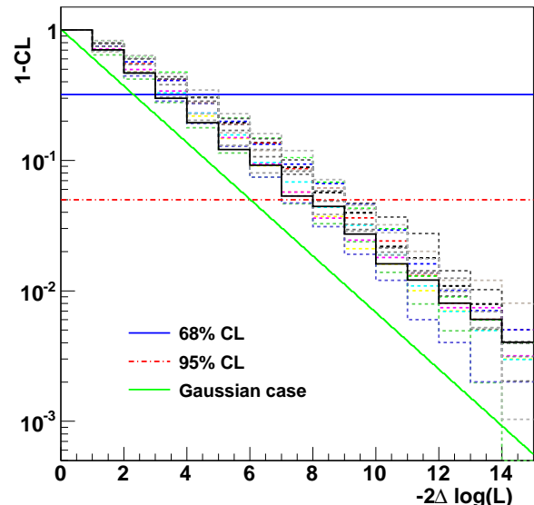
FIG. 14. (color online). Mapping of p -value ( 1 - \text{C.L.} ) as a function of twice the negative difference of log-likelihoods ( -2\Delta\log\mathcal{L} ) as evaluated in pseudoexperiments. The ideal dependence is a \chi^2 distribution with two degrees of freedom as shown by the solid (green) line. The actual observed mapping for our data is shown by the black histogram, while the corresponding distributions for the alternative ensembles are displayed by the colored, dashed histograms.
