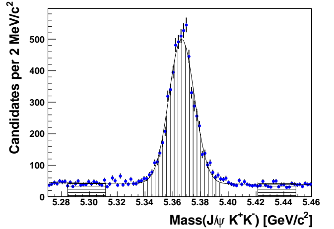
FIG. 5. J/\psi K^+ K^- invariant mass distribution with a cut of 0.2 on the ANN discriminant (left) and in addition with a lifetime requirement ct > 60 \mu\text{m} on the B_s^0 candidate (right). The areas with vertical (horizontal) lines indicate the signal (sideband) regions used in Sec. VI.
