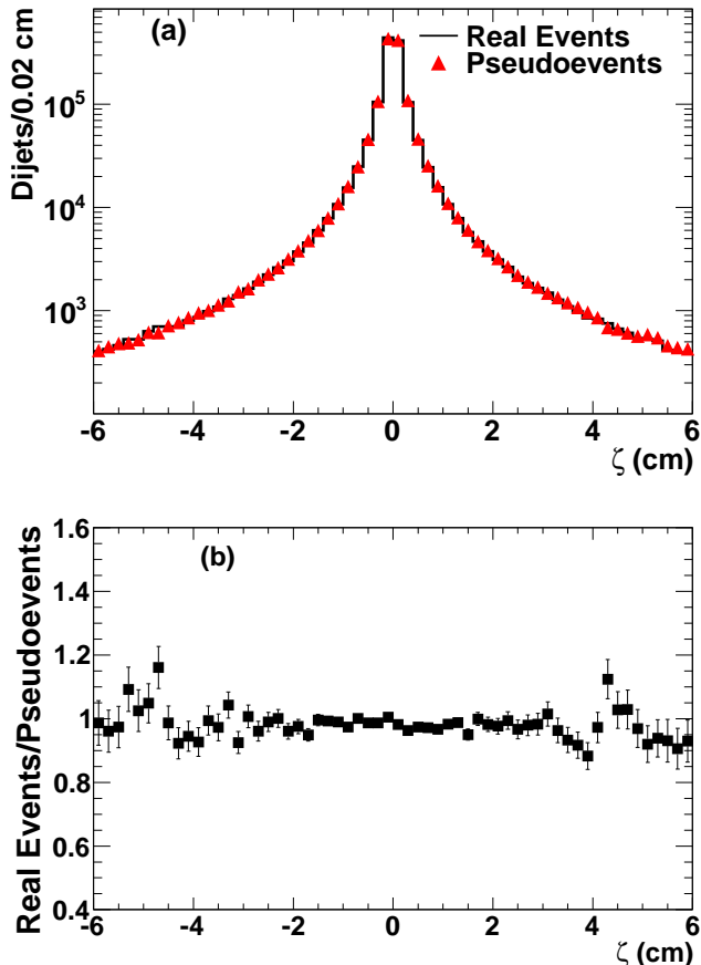
FIG. 7: The distribution of \zeta for the real events (solid line) and pseudoevents (triangle points) in the control region (a), and their ratio (b).
