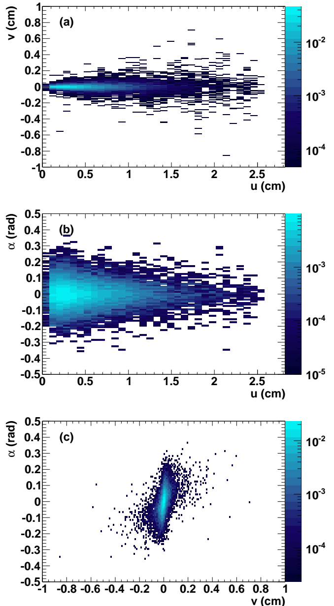
FIG. 5: Two-dimensional projections of a b -quark pdf for jets with E_T from 30 to 70 GeV and one SVT track within the jet: (a) u vs. v , (b) \alpha vs. u , and (c) \alpha vs. v .
