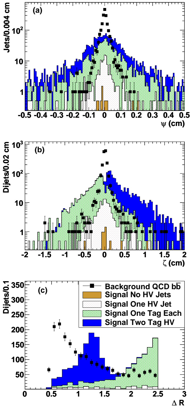
FIG. 4: Distributions of (a) \psi , (b) \zeta , and (c) \Delta R for dijets where both jets are tagged. The signal MC simulation histograms are stacked. In (a), only the leading jet of the jet pair is shown. In (c), a \Delta R < 2.5 cut has already been applied.
