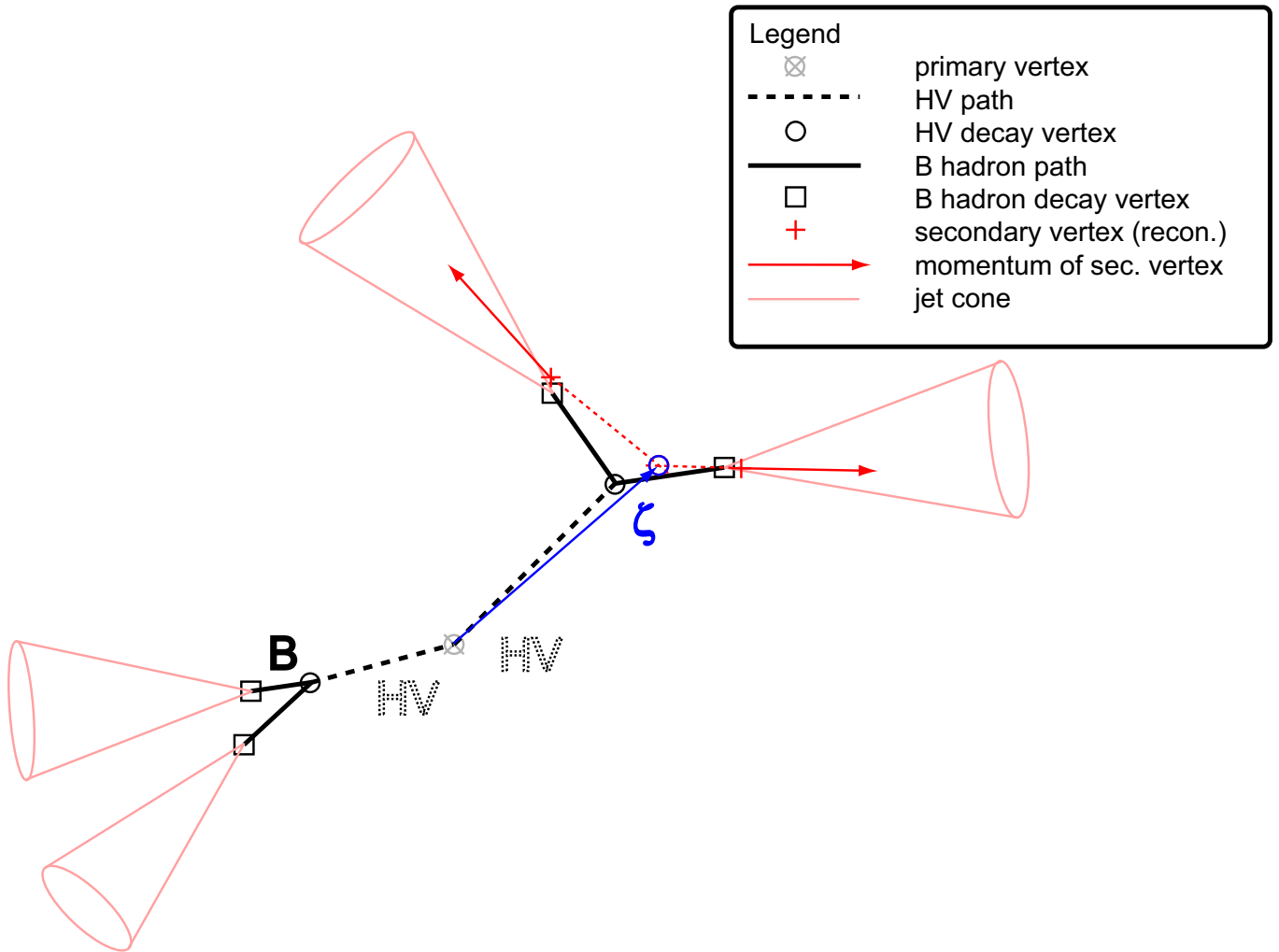
FIG. 3: Schematic diagram of variable \zeta , which represents the decay vertex of the HV particle.
