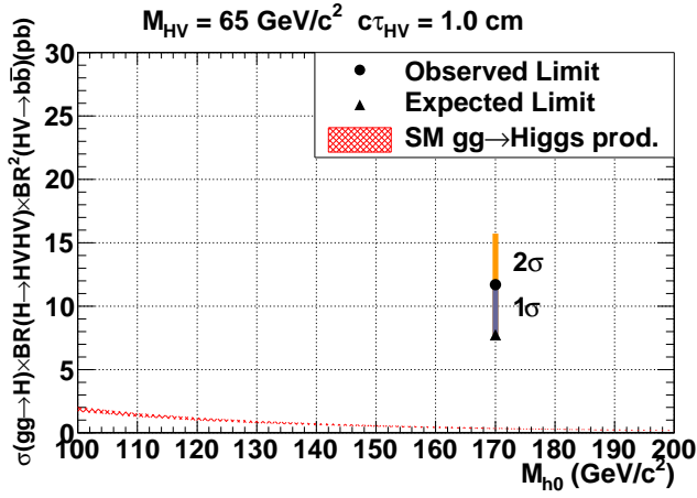
FIG. 11: Observed and expected limits at 95% C.L. with +1 and +2 \sigma bands for signal MC with HV masses 65 \text{GeV}/c^2 . The hashed line is the Higgs boson production cross section in the SM.
