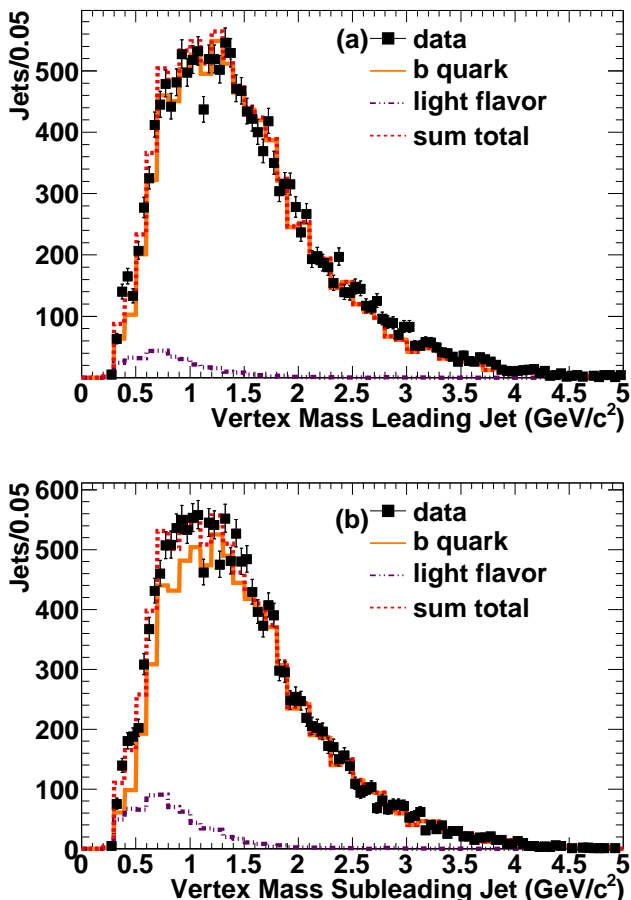
FIG. 6: Example of double-flavor fits for dijets where each jet has exactly one SVT trigger track. Histograms are projections of the two-dimensional fit onto the axis of each jet: (a) the higher E_T jet in the event, (b) the lower E_T jet.
