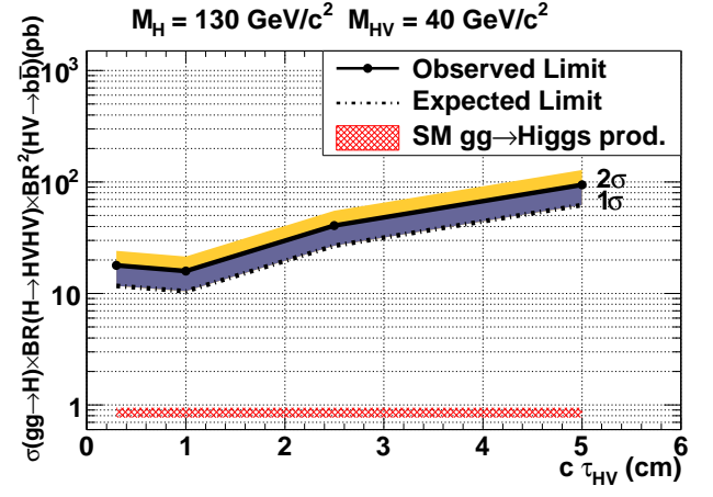
FIG. 12: Observed and expected limits at 95% C.L. with +1 and 2 \sigma bands for signal MC for differing HV particle lifetimes. The hashed line is the Higgs boson production cross section in the SM.
