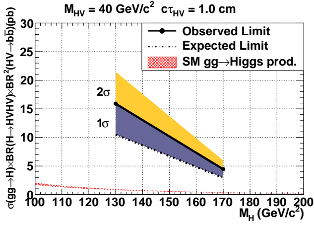
FIG. 10: Observed and expected limits at 95% C.L. with +1 and +2 \sigma bands for signal MC with HV masses 40 \text{GeV}/c^2 . The hashed line is the Higgs boson production cross section in the SM.
