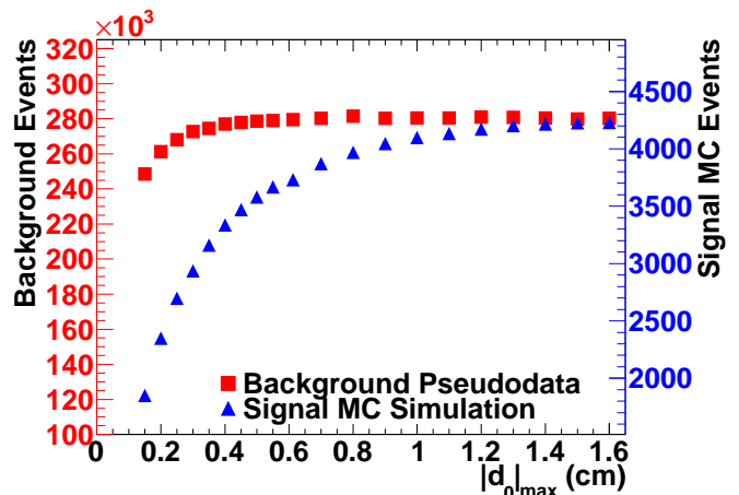
FIG. 8: Number of signal MC simulation events (triangle points) and background pseudoevents (square points) vs. the b -tagging algorithm cut |d_0|_{max} .
