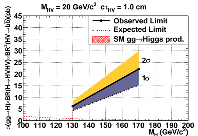
FIG. 9: Observed and expected limits at 95% C.L. with +1 and +2 \sigma bands for signal MC simulation with HV mass 20 \text{GeV}/c^2 . The hashed line is the Higgs boson production cross section in the SM.
