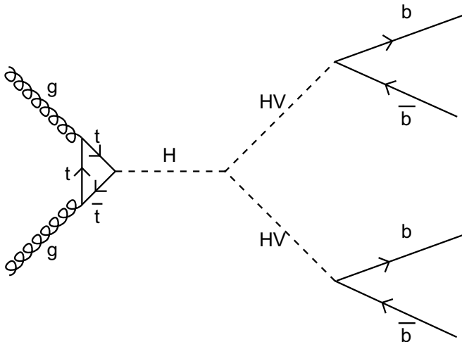
FIG. 1: Feynman diagram of Higgs boson production of a hidden valley (HV) particle and its subsequent decay. The coupling of HV particle to b\bar{b} is extremely small, resulting in the long lifetime.
