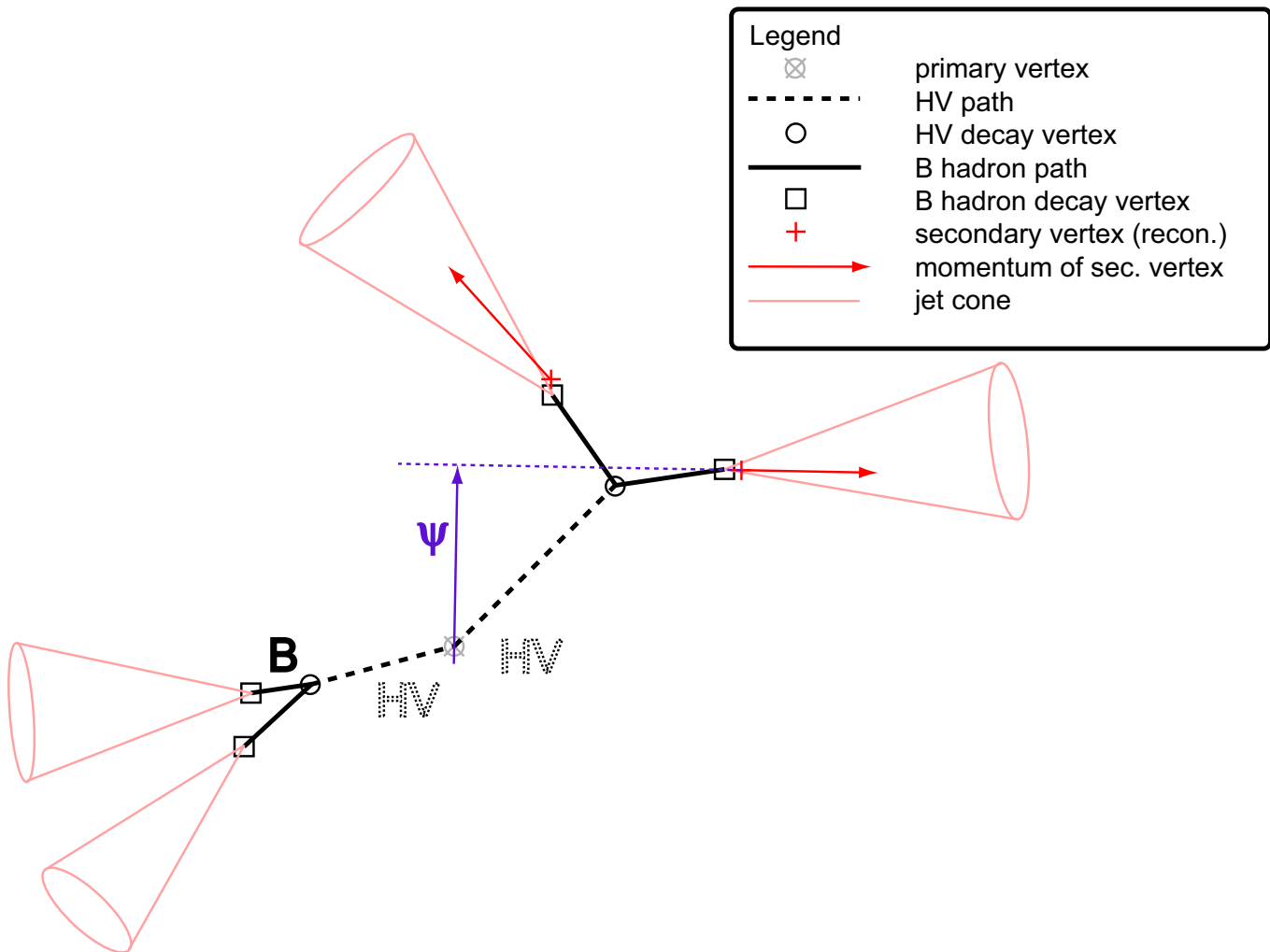
FIG. 2: Schematic diagram of variable \psi , the impact parameter of a jet with a secondary vertex. This figure is not to scale. The figure is shown in a plane transverse to the beamline.
